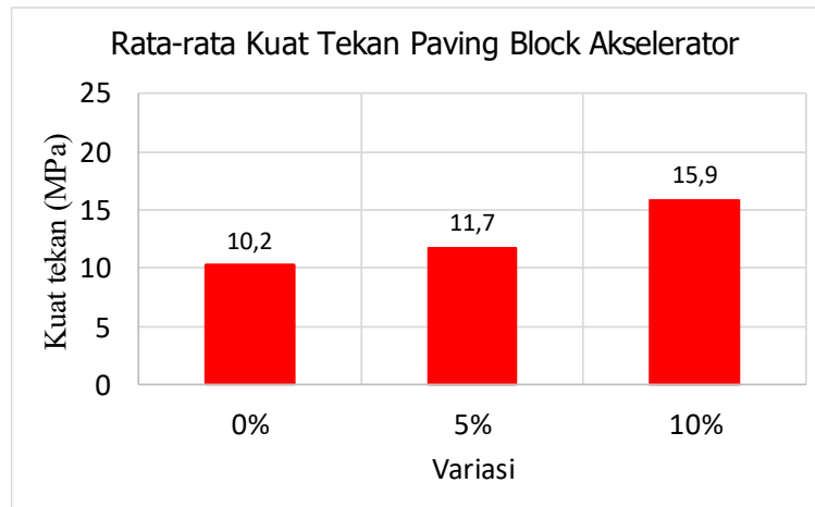
Gambar 4.3. Grafik rata-rata kuat tekan paving block akselerator
