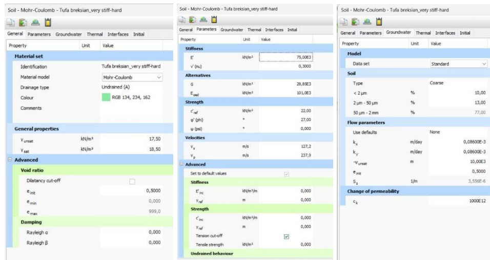
Gambar 4.4 Material Setting Lempung Lanauan_very stiff-hard
