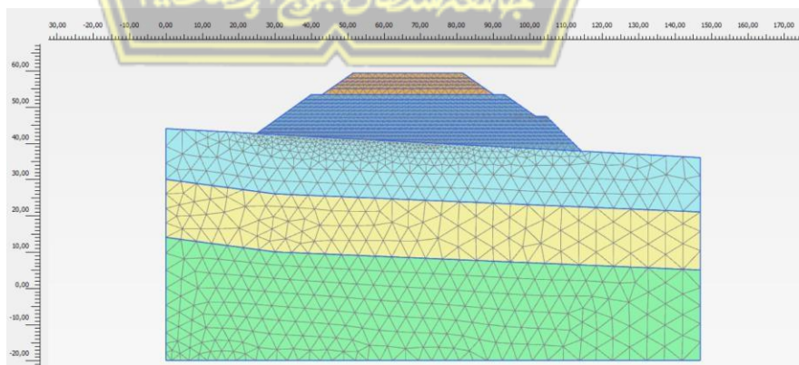
Gambar 4.16 Output Mesh
