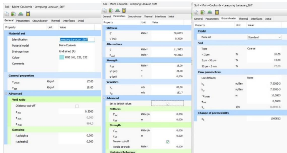
Gambar 4.2 Material Setting Lempung Lanauan_very soft
