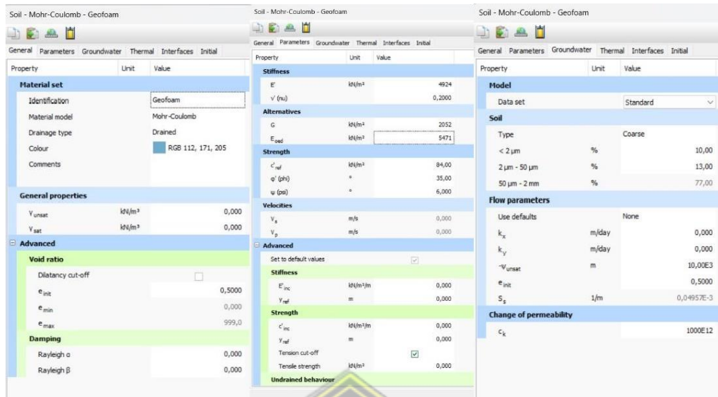
Gambar 4.6 Material Setting Geofoam
