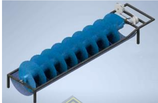
Gambar 4. 2 Desain 3D PLTMH tipe turbin archimedes screw.
