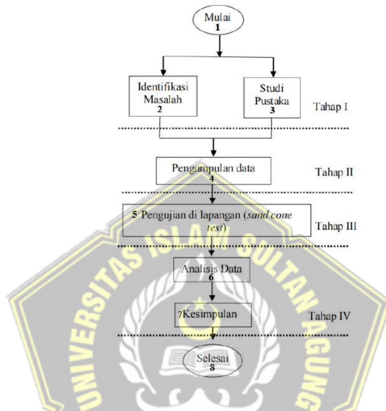
Gambar 3.2 Diagram Alir
