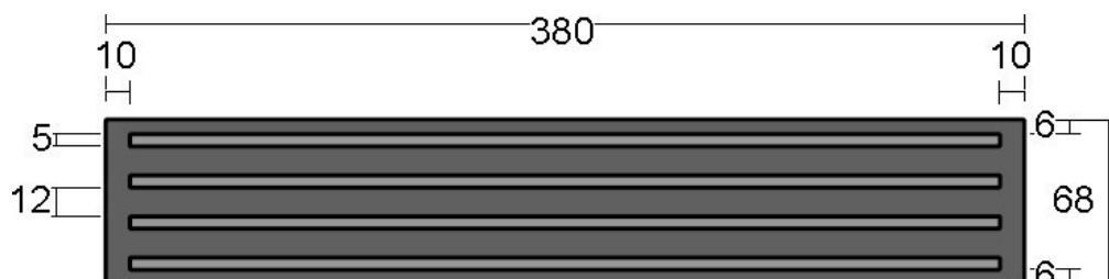
Gambar 4. 28 Gambar Rencana Elastomeric Bearing Pad
