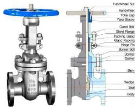
Gambar 2.2 Gate Valve
