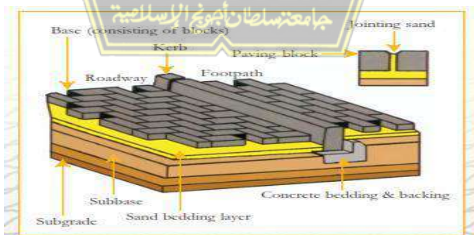
Gambar 2.14 Lapisan Perkerasan Paving Block (Tsani, (2019)
