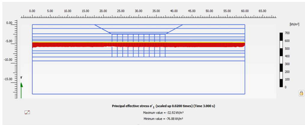
Gambar 4.32 \sigma^I lapisan loose sand tanah asli
