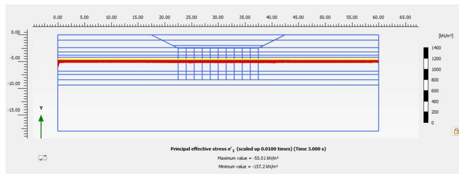
Gambar 4.24 Principal Effective Stress \sigma^I lapisan loose sand RI
