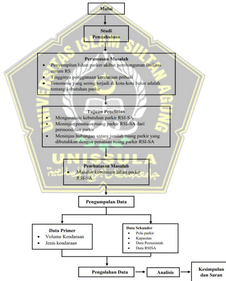
Gambar 3.1. Alur Penelitian
