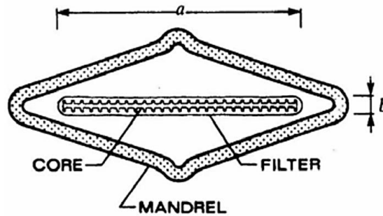
Gambar 2.15 Diameter Equivalen ( d_w ) untuk Prefabricated Vertical Drain (PVD) (Mochtar, 2012)
