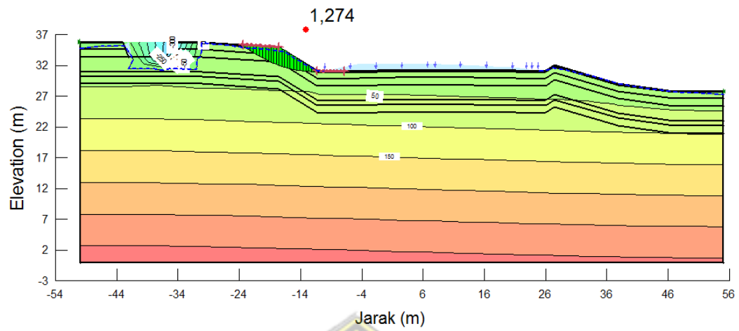
Gambar 4. 44 Nilai SF Curah Hujan Serpan 2016
