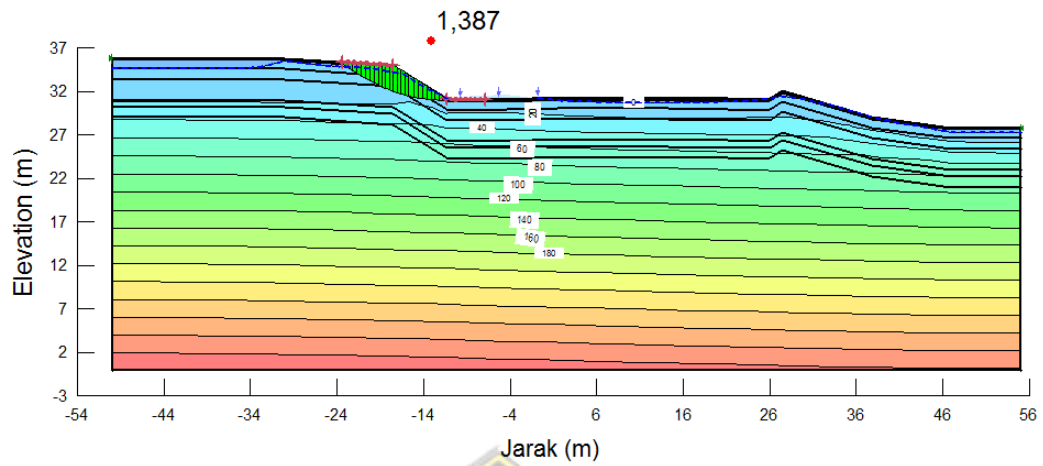
Gambar 4. 36 Nilai SF Curah Hujan Serpan 2016
