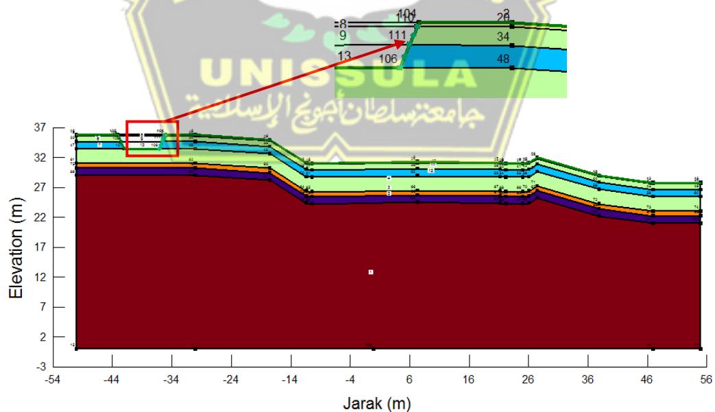
Gambar 4. 27 Permodelan Penambahan Seepage
