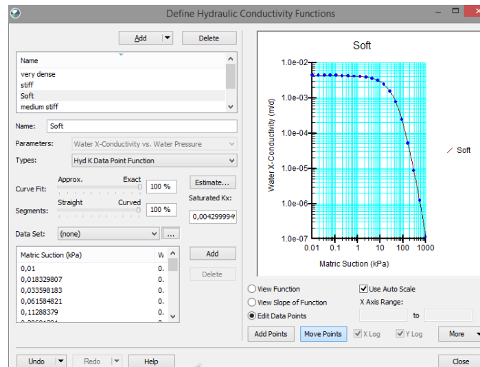
Gambar 4. 15 Define hydraulic Conductivity
