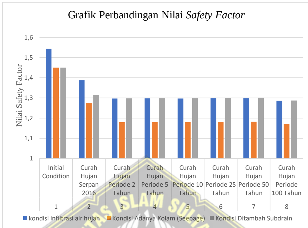
Gambar 4. 59 Grafik Nilai Safety Factor
