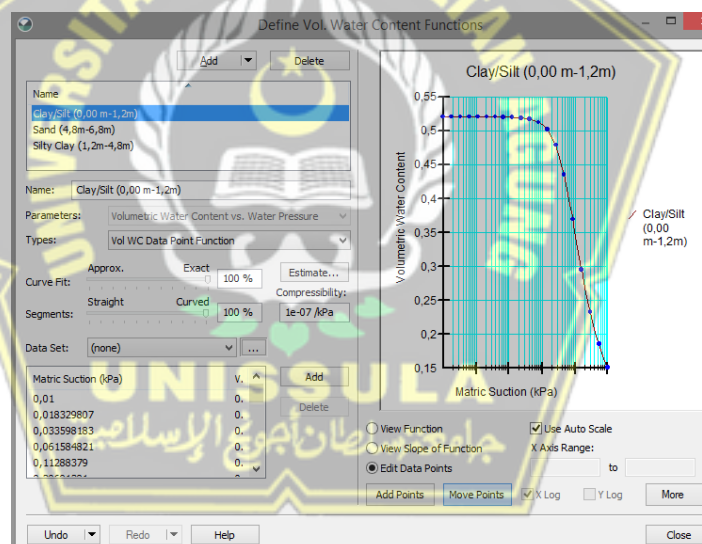
Gambar 4. 16 Vol Water Content functions
