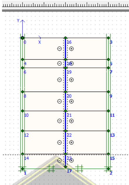
Gambar 4.8 Model geometri penampang Melintang Jepit Standar ( Standard Fixties )
