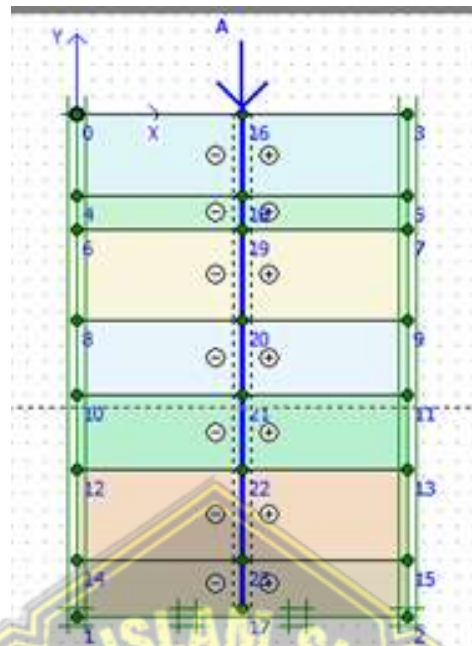
Gambar 4.14 Geometri penampang
