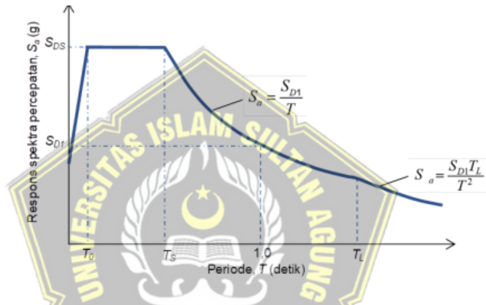
Gambar 2.3 Spektrum Respons S_a (SNI 1726 : 2017)
