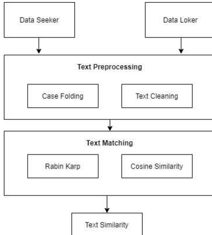
Gambar 3.1: Metode Penelitian
