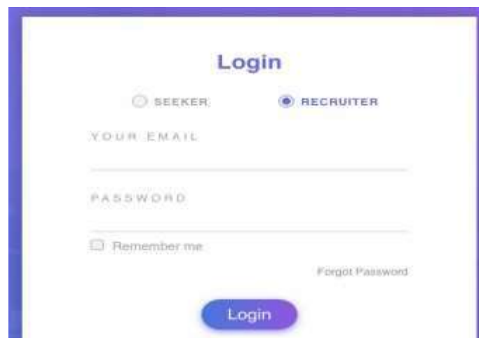
Gambar 4.8: Login Recruiter
