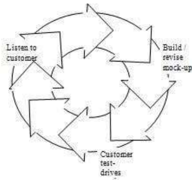
Gambar 3.1 Model Prototyping
