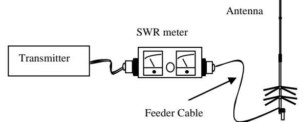
Fig. 4 Characteristics Frequency Antenna Measurement Model
