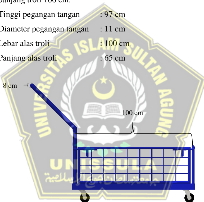
Gambar 1. Tampak Samping
