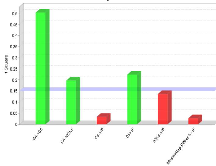
f Square
