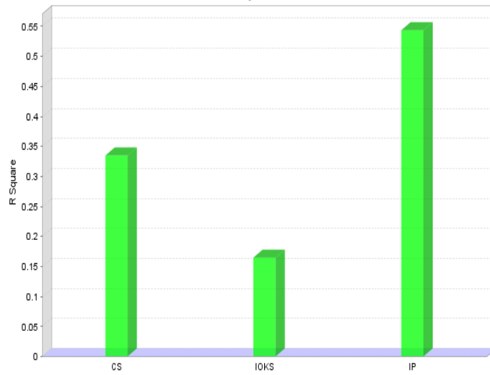
R Square
