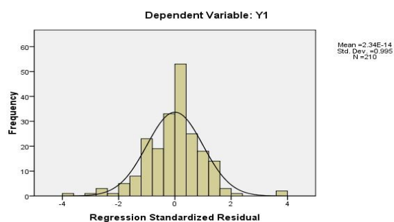
Histogram
