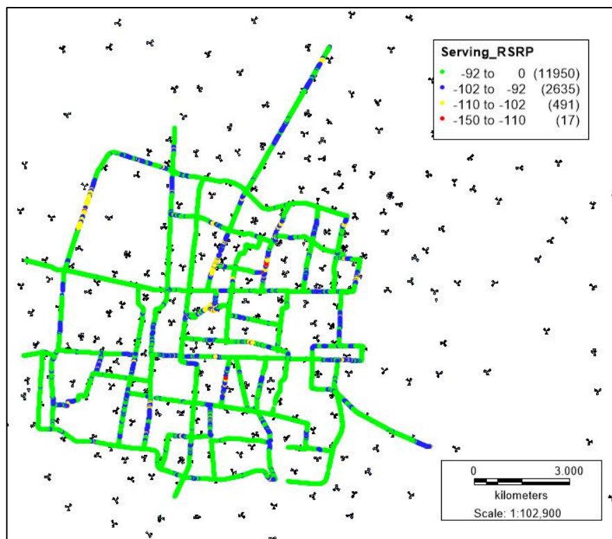
Gambar 4 Tampilan RSRP Data Plotting April 2018
