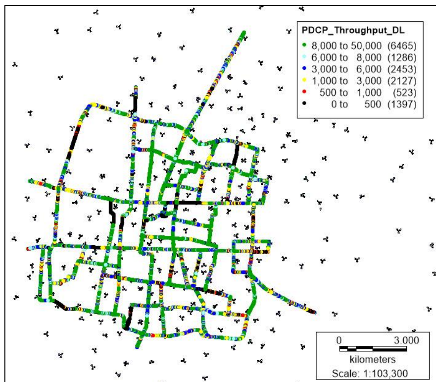
Gambar 20 Tampilan PDCP Throughput Download Data Plotting Juni 2018
