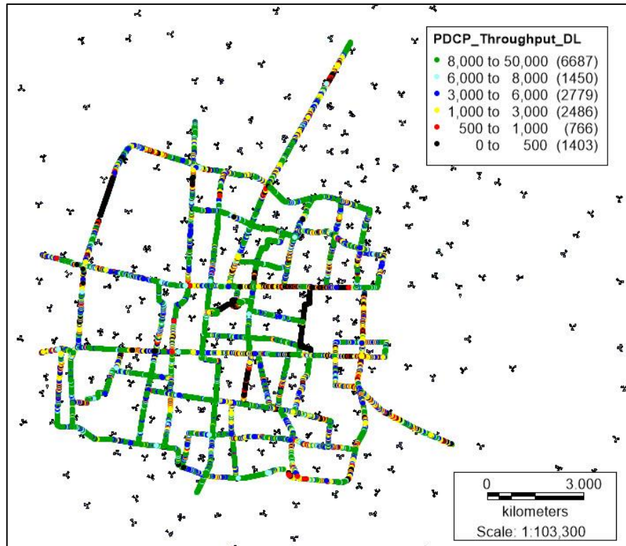
Gambar 19 Tampilan PDCP Throughput Download Data Plotting Mei 2018
