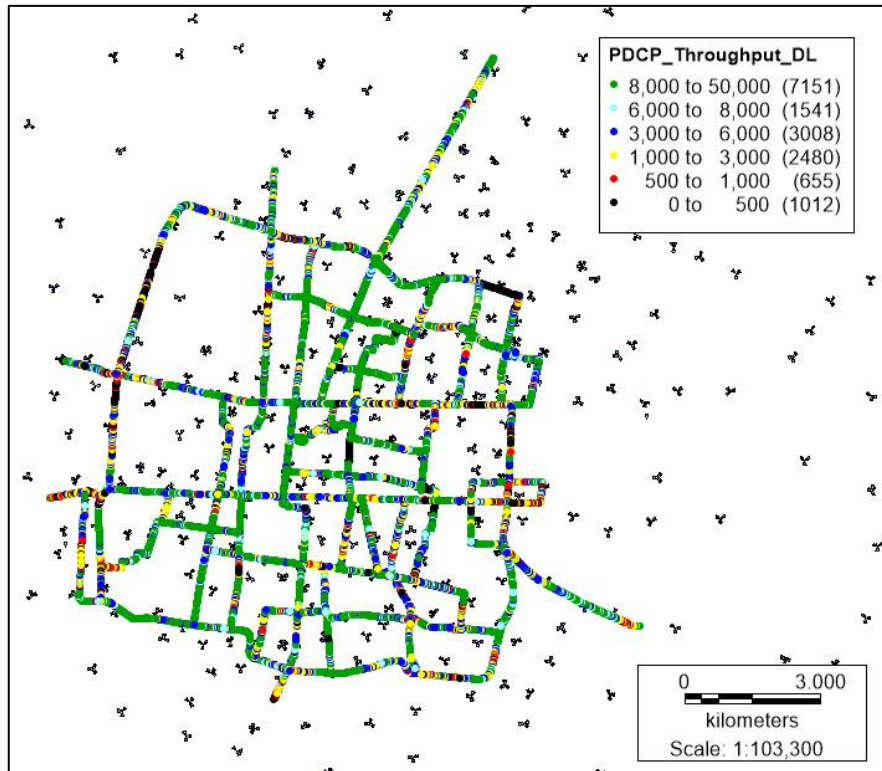
Gambar 17 Tampilan PDCP Throughput Download Data Plotting Maret 2018
