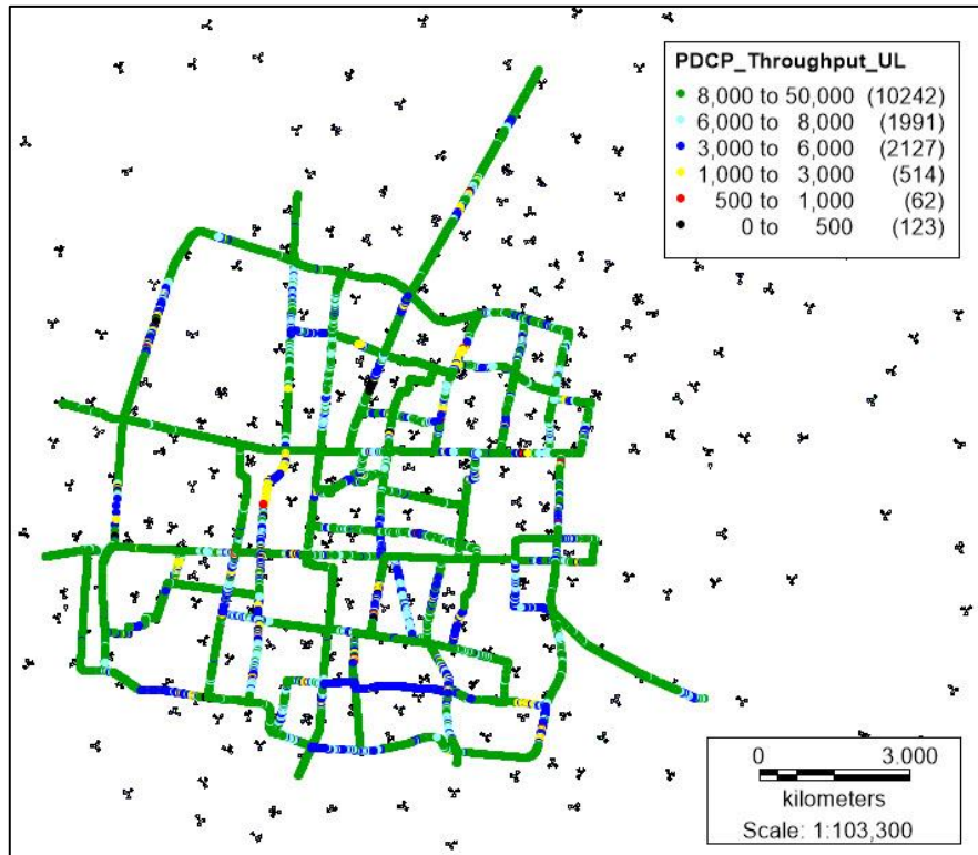
Gambar 26 Tampilan PDCP Throughput Upload Data Plotting Mei 2018
