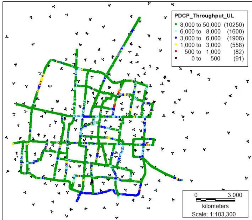
Gambar 28 Tampilan PDCP Throughput Upload Data Plotting Juli 2018
