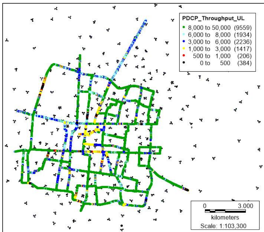
Gambar 25 Tampilan PDCP Throughput Upload Data Plotting April 2018
