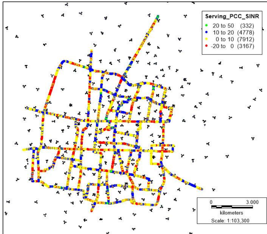
Gambar 10 Tampilan SISR Data Plotting Maret 2018
