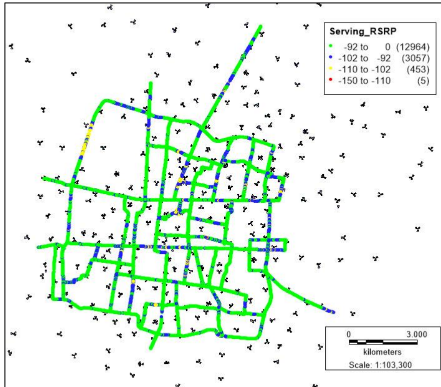
Gambar 3 Tampilan RSRP Data Plotting Maret 2018
