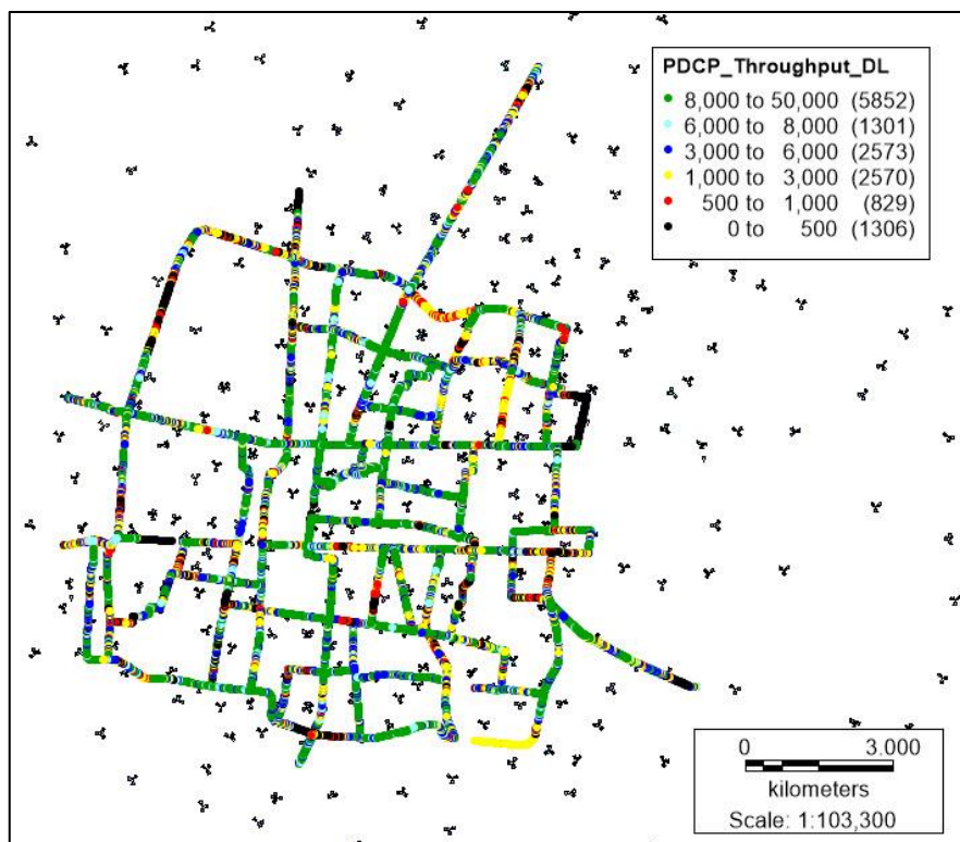
Gambar 18 Tampilan PDCP Throughput Download Data Plotting April 2018
