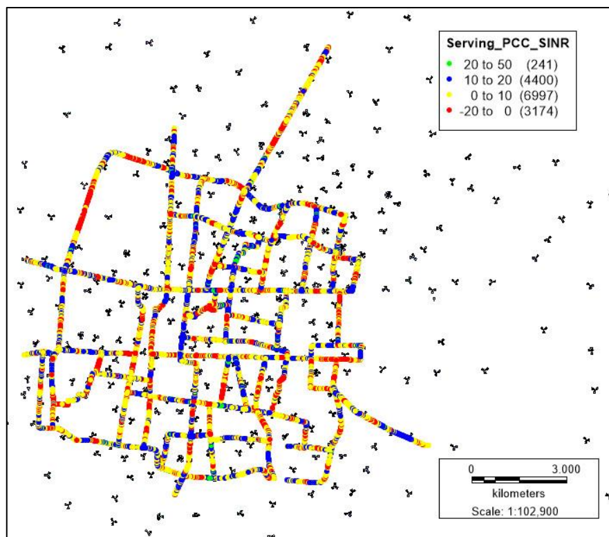
Gambar 11 Tampilan SISR Data Plotting April 2018
