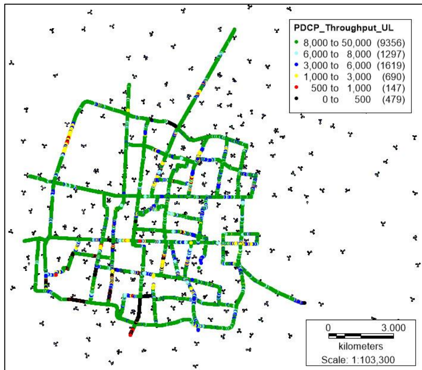
Gambar 23 Tampilan PDCP Throughput Upload Data Plotting Februari 2018
