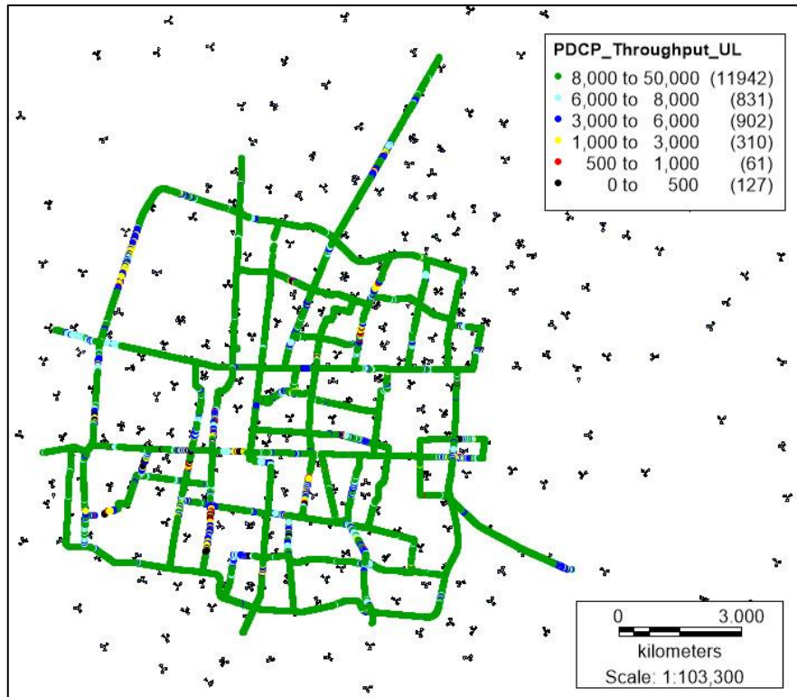
Gambar 24 Tampilan PDCP Throughput Upload Data Plotting Maret 2018
