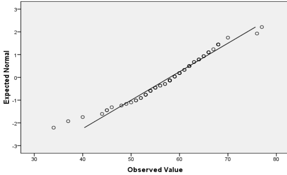
Normal Q-Q Plot of Usia
