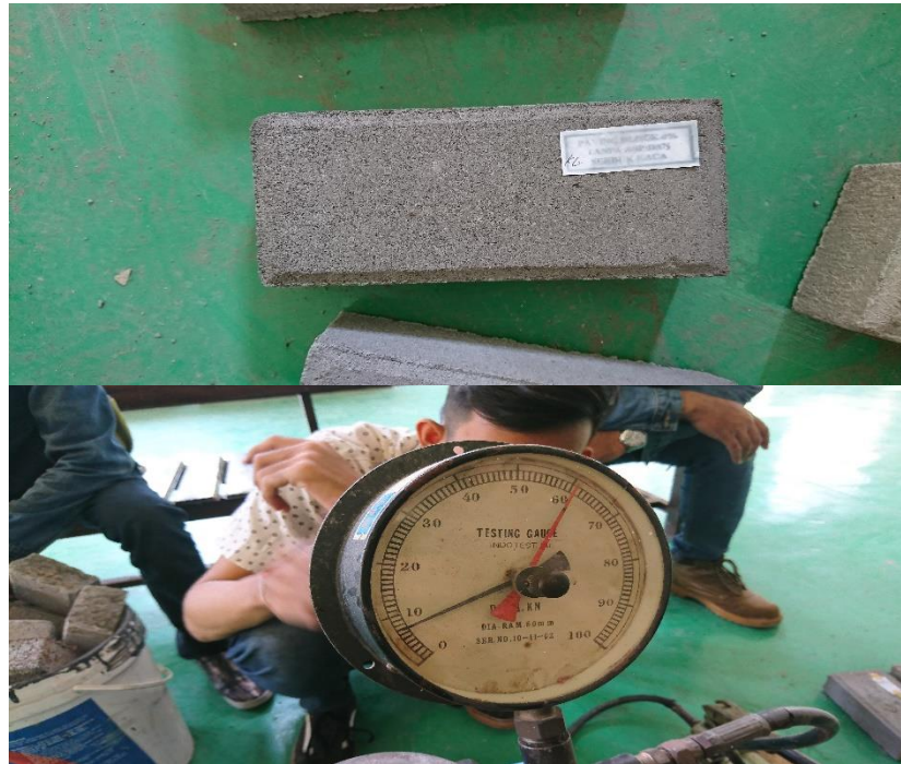
Gambar 32. Uji Kuat Lentur Cone Block Normal
