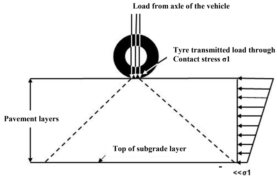
Figure 1.2. Load distributions on flexible pavement
