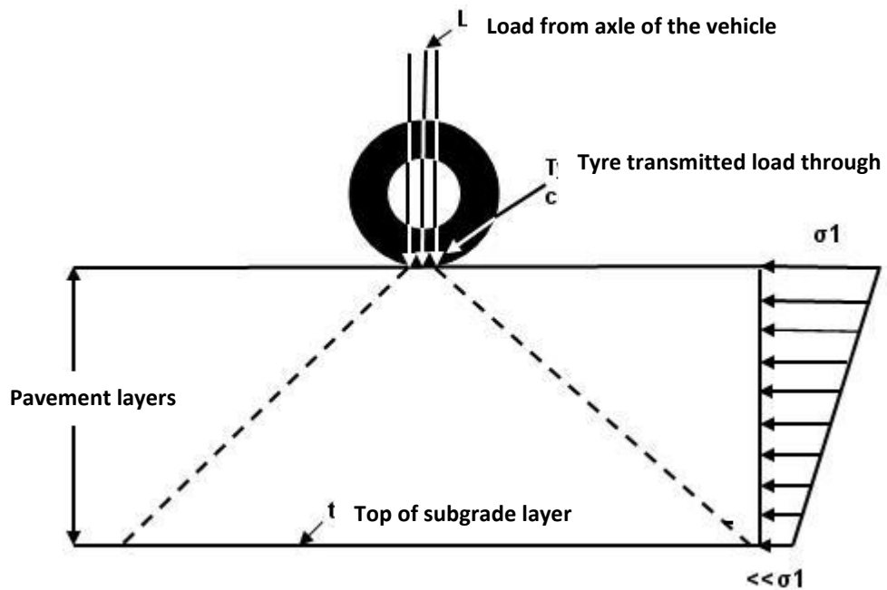
Figure 1.2: Load distributions on flexible pavement
